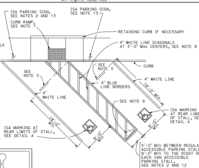
DIAGONAL DOUBLE PARKING STALLS
