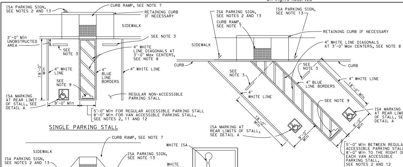
DIAGONAL DOUBLE PARKING STALLS
