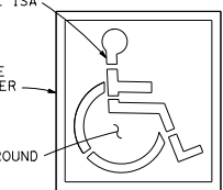
ISA MARKING See Revised Std Plan RSP A24C
