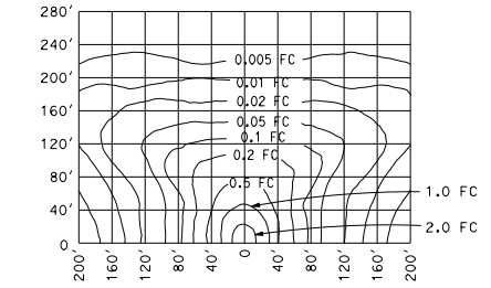
LOW-PRESSURE SODIUM LUMINAIRE 180 W 40' Mounting Height Lamp operated at 33,000 lm
