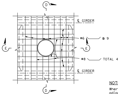
PART PLAN
