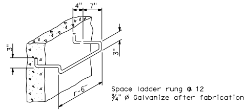
BAR STEP LADDER RUNG DETAILS DETAIL U44
