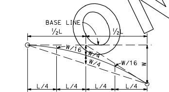
TYPICAL PARABOLIC LAYOUT
