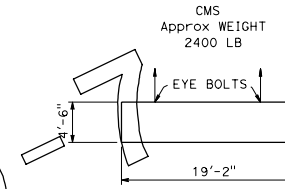
LIFTING DIAGRAM
