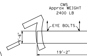
LIFTING DIAGRAM
