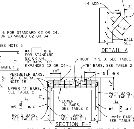
SECTION F-F
