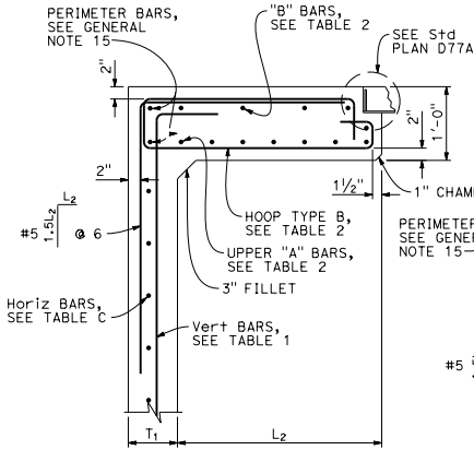
SECTION G-G
