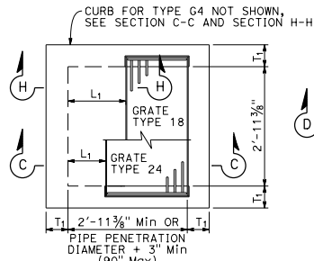
PLAN STANDARD TYPE G2 OR G4
