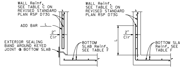
BASE WITH KEYED JOINT INTEGRAL BASE
