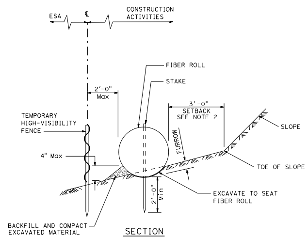
SECTION PLACEMENT DETAIL FOR TEMPORARY HIGH-VISIBILITY FENCE USED WITH TEMPORARY LARGE SEDIMENT BARRIER (See Note 1)
