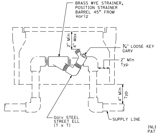
ELEVATION WYE STRAINER ASSEMBLY
