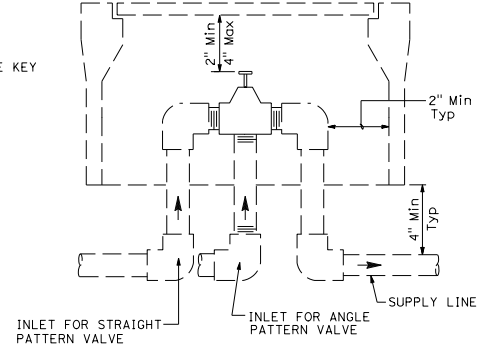
ELEVATION VALVE
