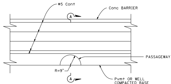
ELEVATION See Notes 1 and 2
