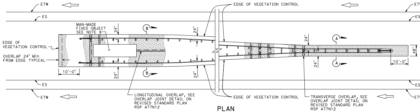
PLAN Fixed object(s) between separate roadbeds (One-Way Traffic)
