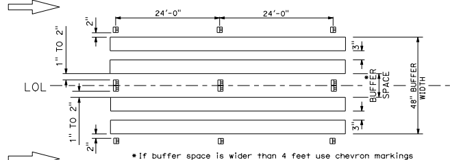
DETAIL 45
