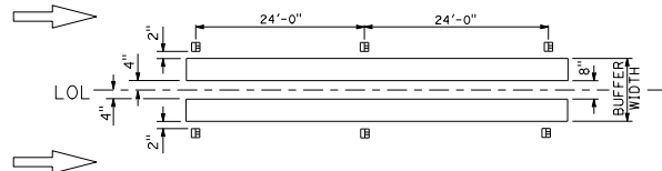
DETAIL 44B
