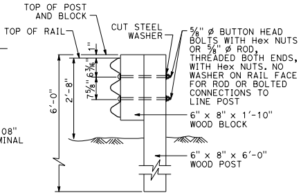
SECTION B-B TYPICAL WOOD LINE POST INSTALLATION
