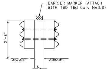
THRIE BEAM BARRIER DELINEATION See Note 8
