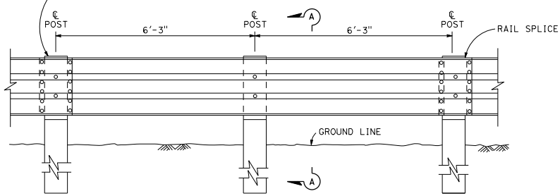
DOUBLE THRIE BEAM BARRIER (Wood post and blocks) See Note 1
