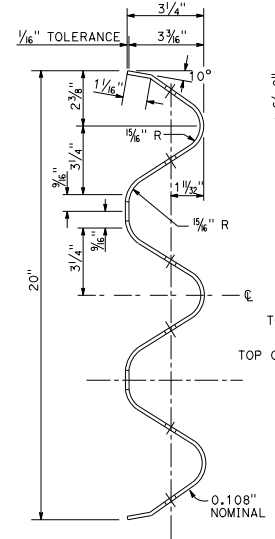
SECTION THRU RAIL ELEMENT
